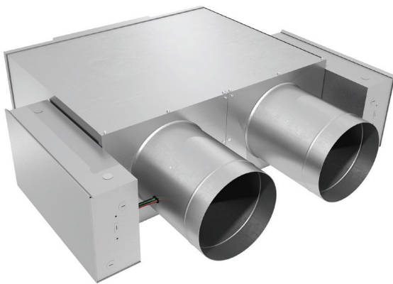
Standard Mixing Dual Duct Terminal Unit
